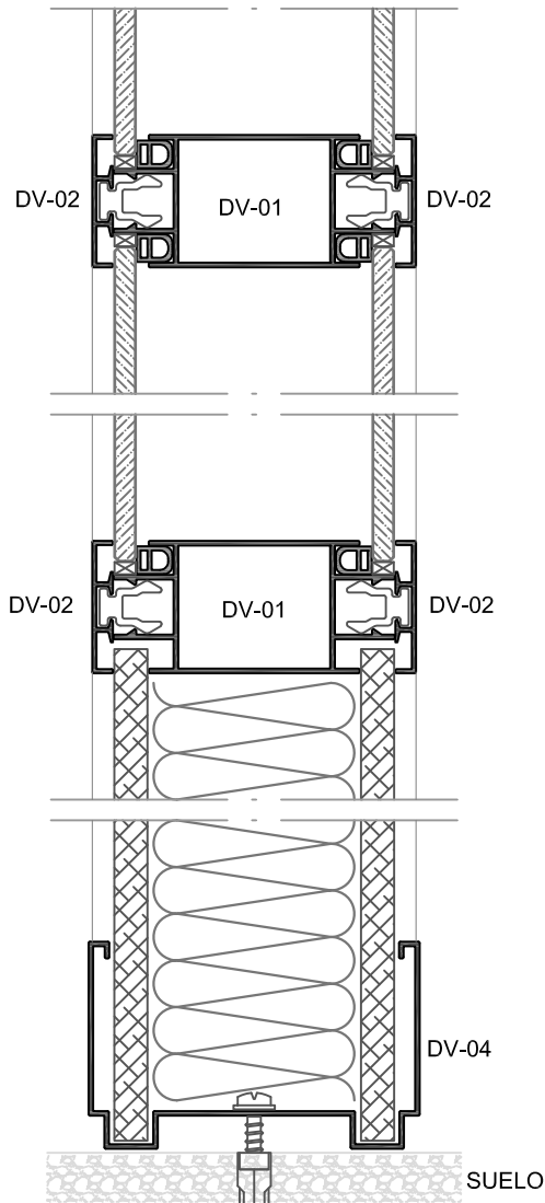
CORTE VERTICAL
